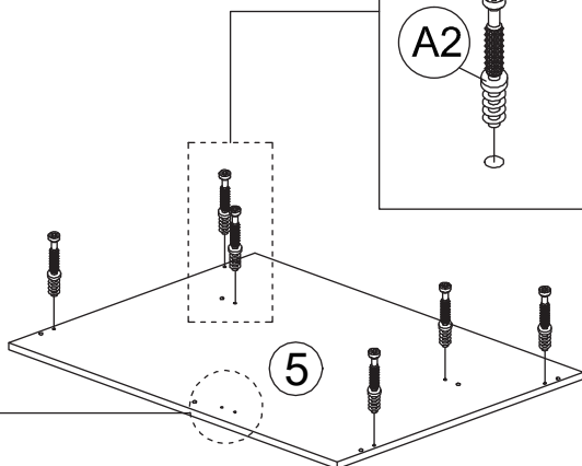
1 BOTTOM VIEW
