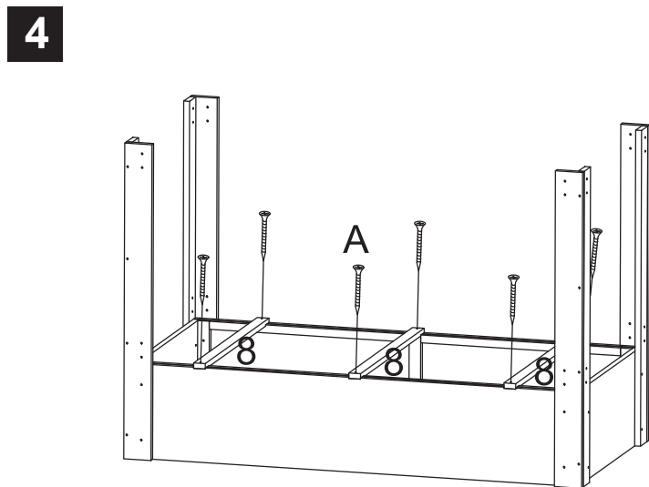
Ax16 M3x30mm
