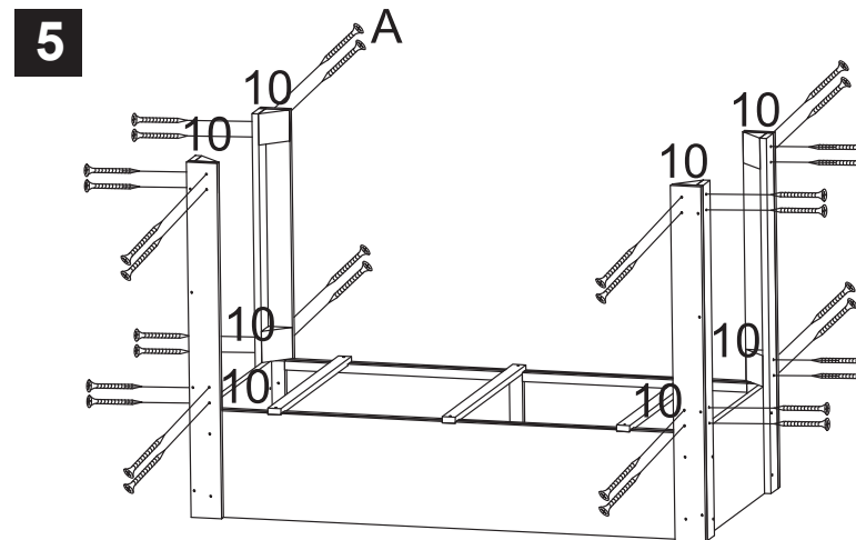
Ax32 M3x30mm
